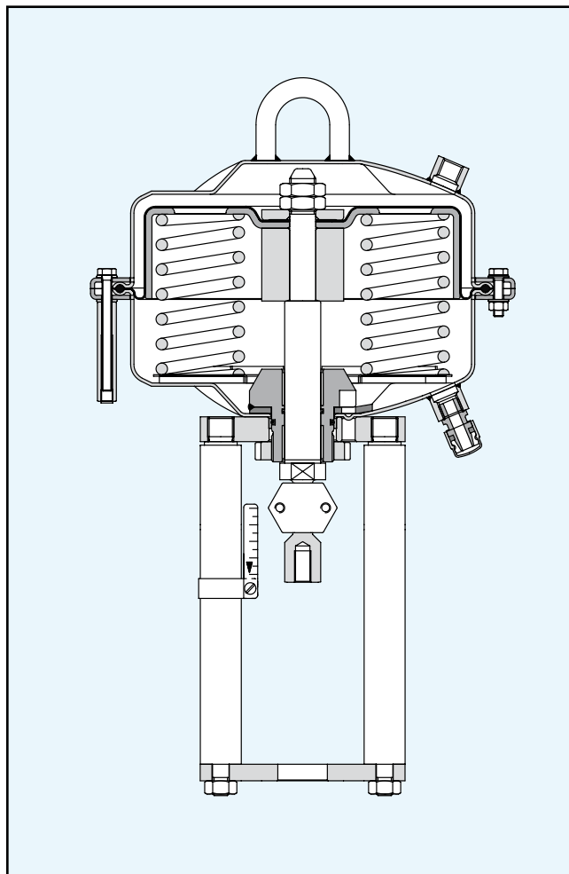
Air-to-Close version
