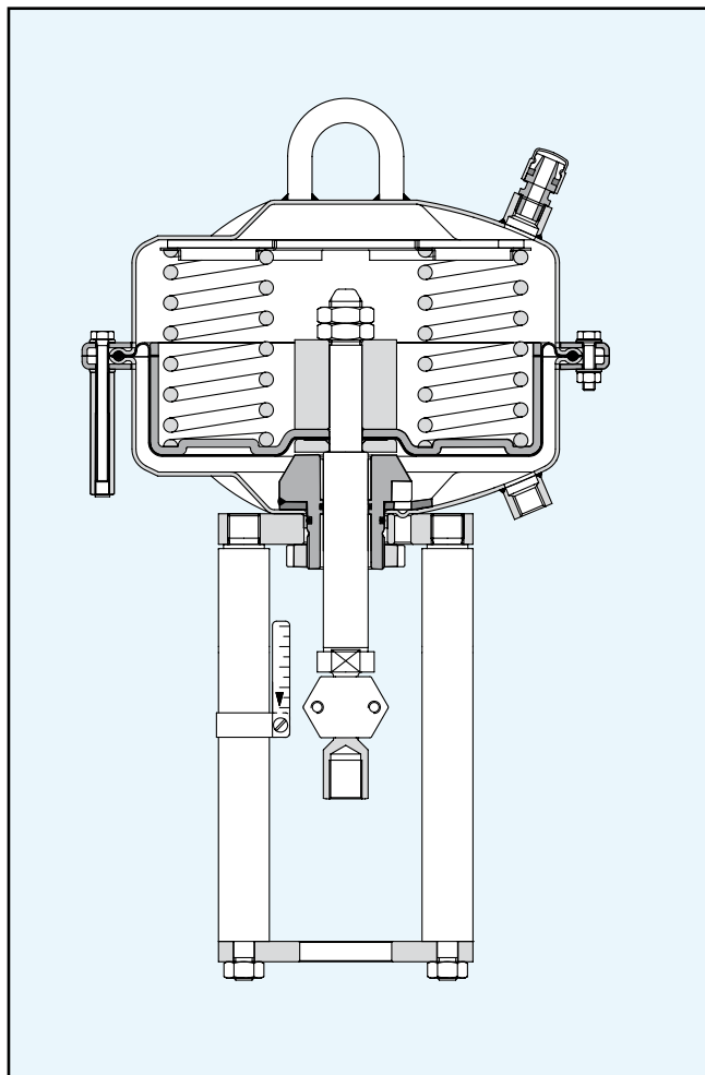
Air-to-Open version
