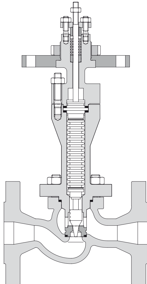
Bellows Seal
