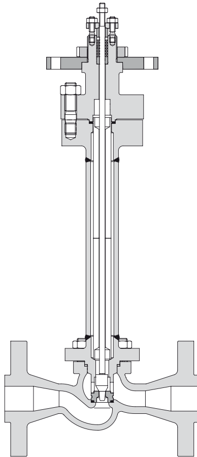
Cryogenic Extension
